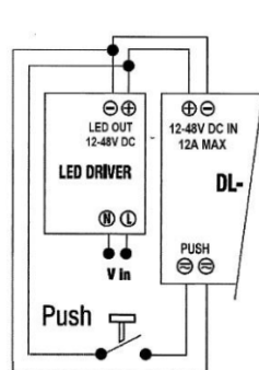
Schema/wiring Push 12-48Vdc
